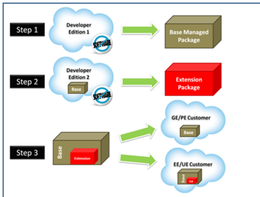
Using a base and extension package to support multiple editions
