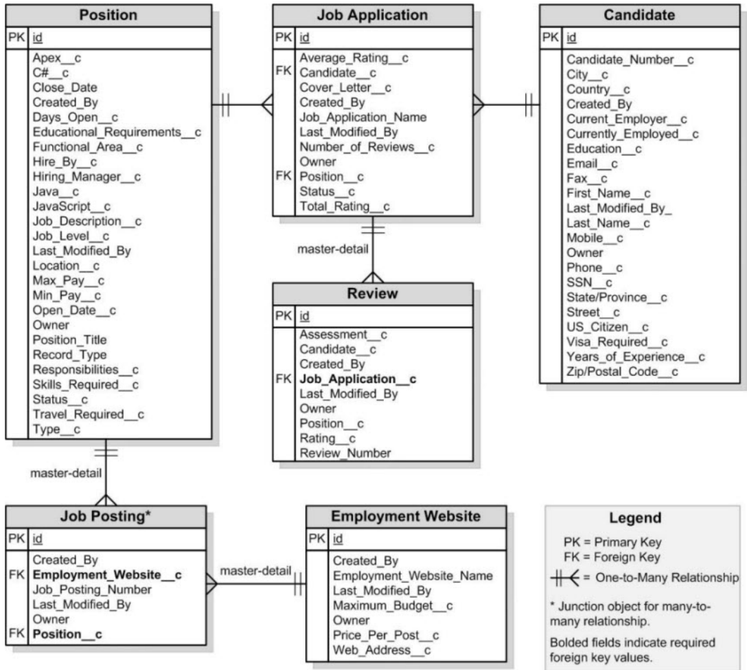
Recruiting App Entity Relationship Diagram
