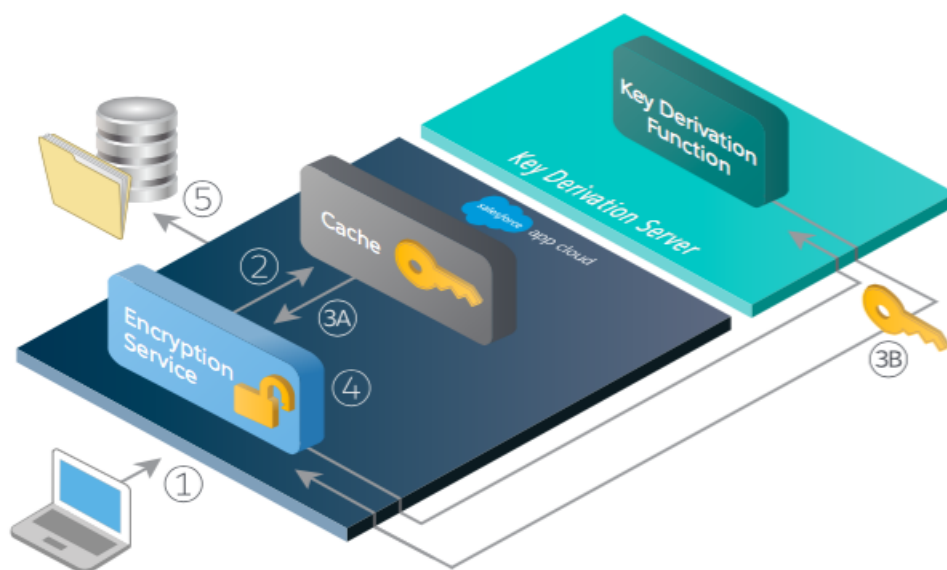
Platform Encryption Process Flow
